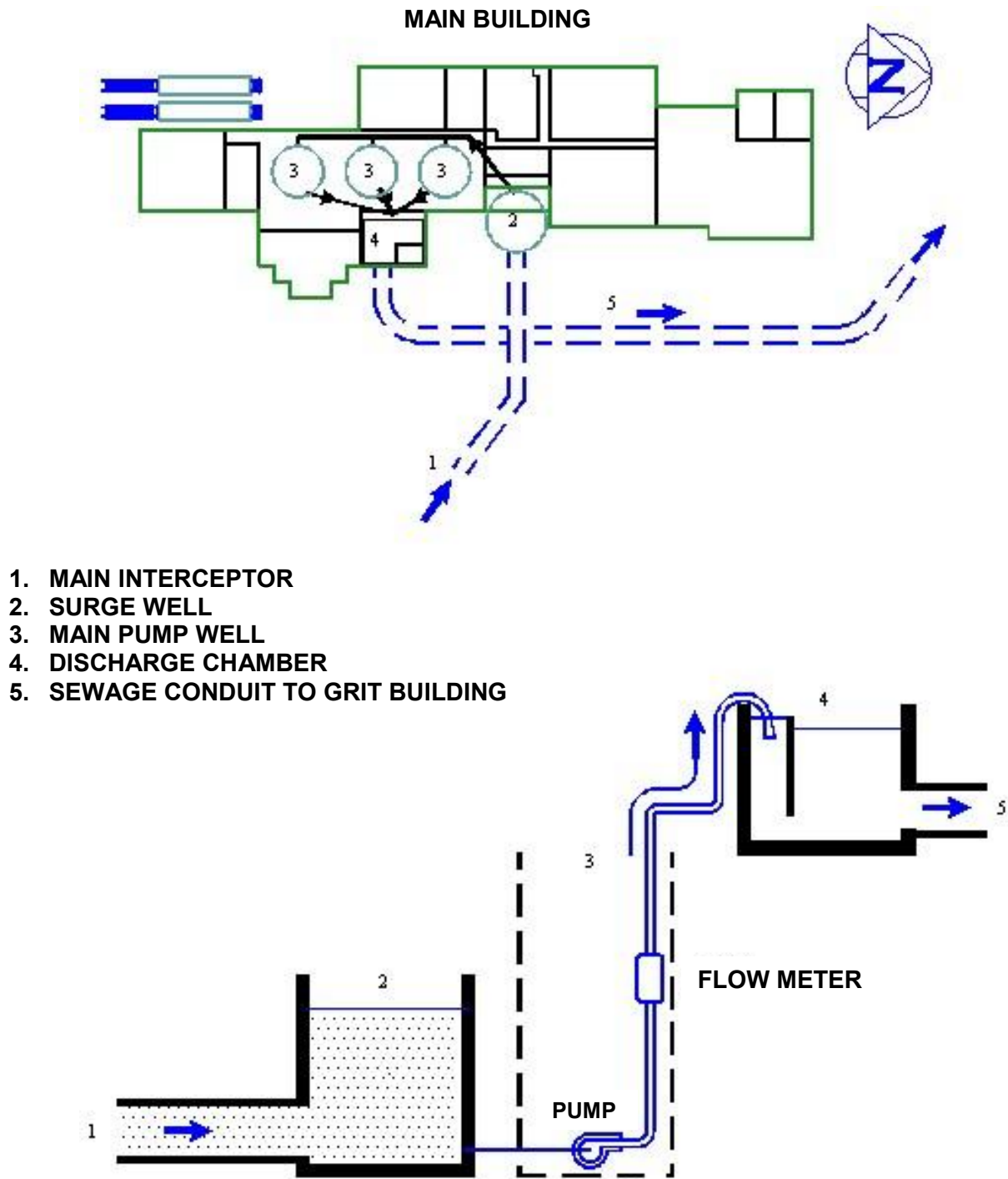
Figure 2. North End Water Pollution Control Centre influent pumping system.
